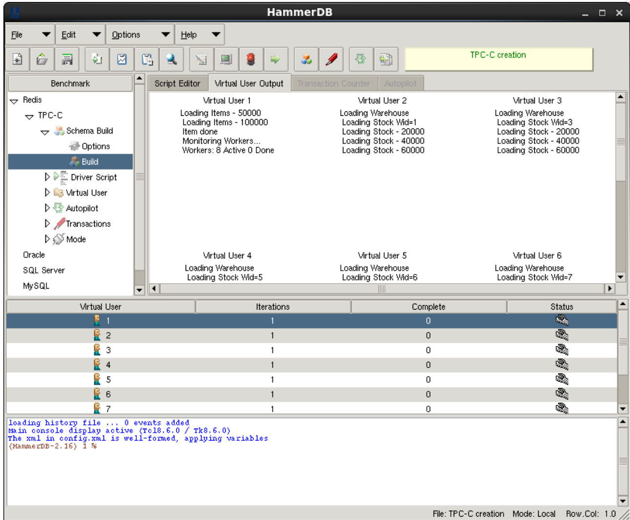
Figure 5 Schema Building
