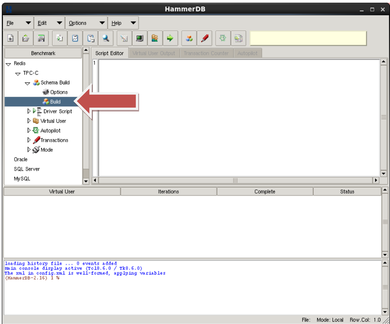
Figure 3 Create Schema
